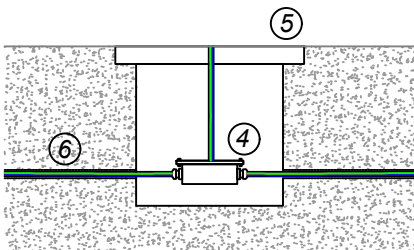
Vista Frontal
