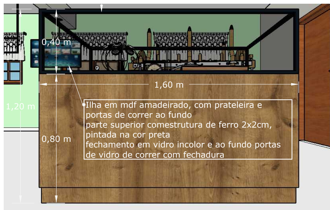
Vista Frontal
