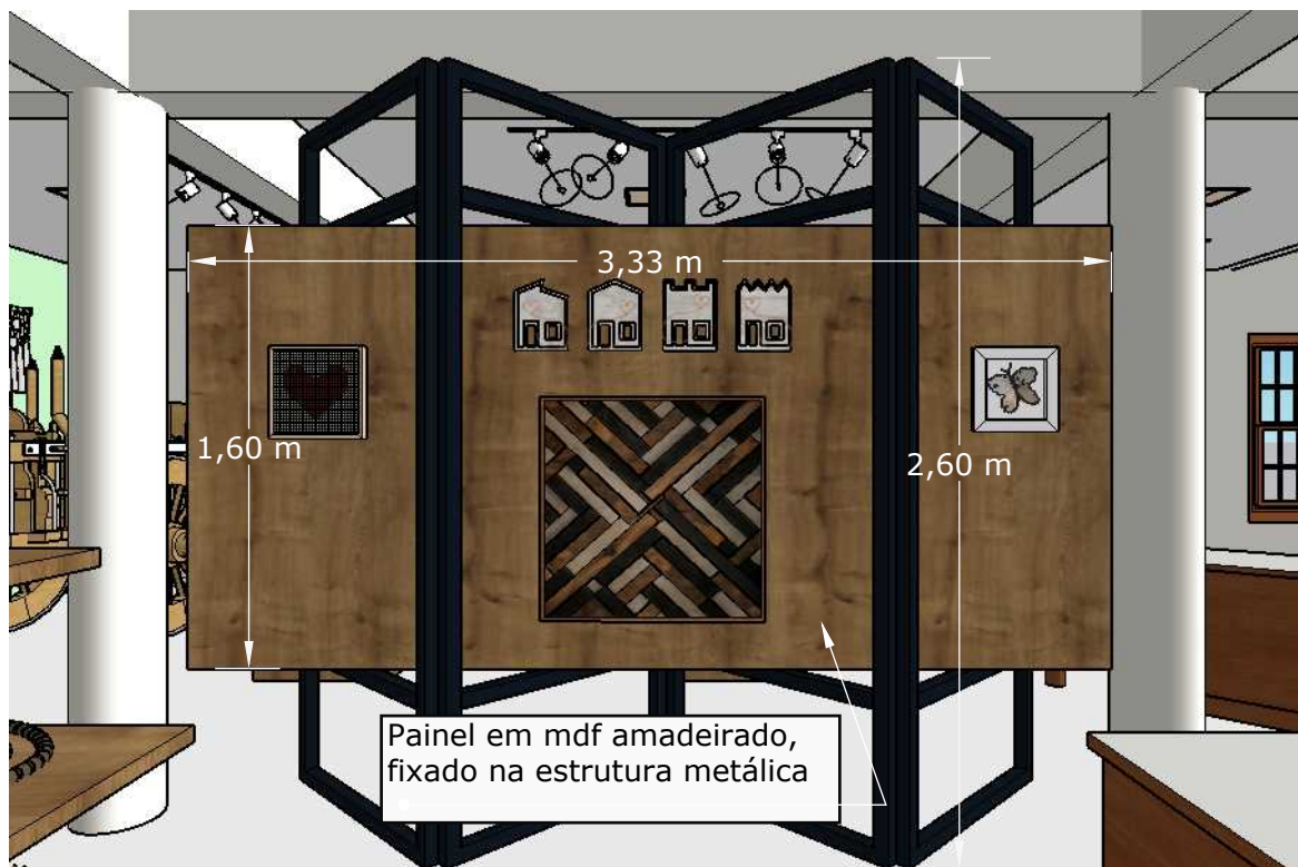
Vista Frontal
