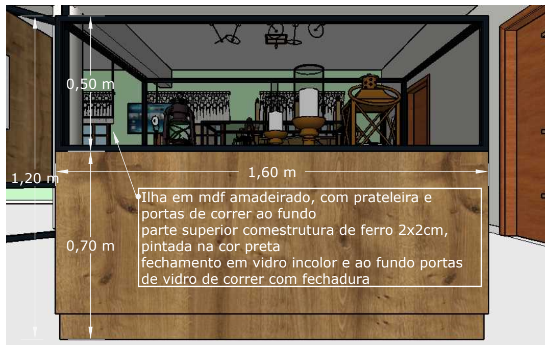
Vista Frontal
