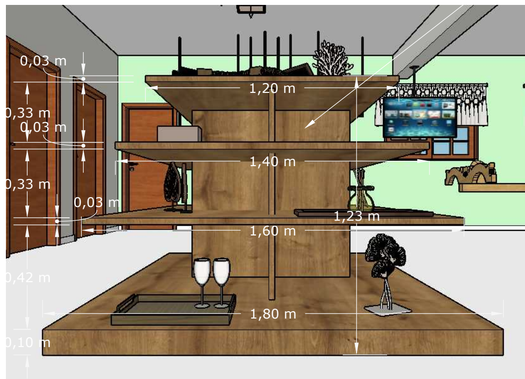
Vista Frontal
