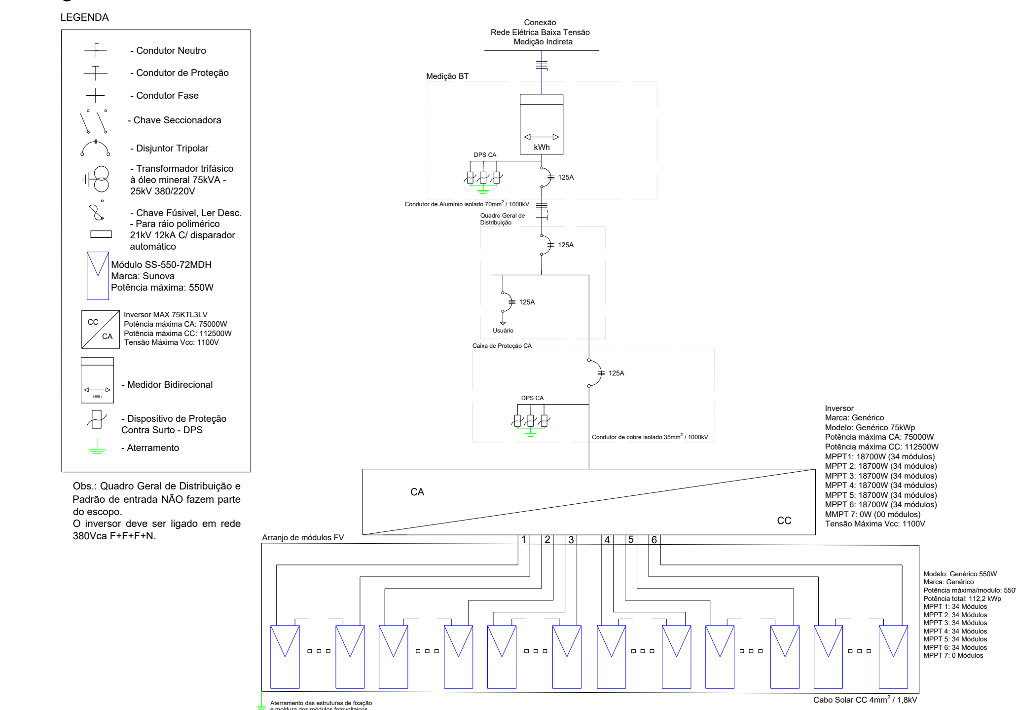
Diagrama Unifilar
