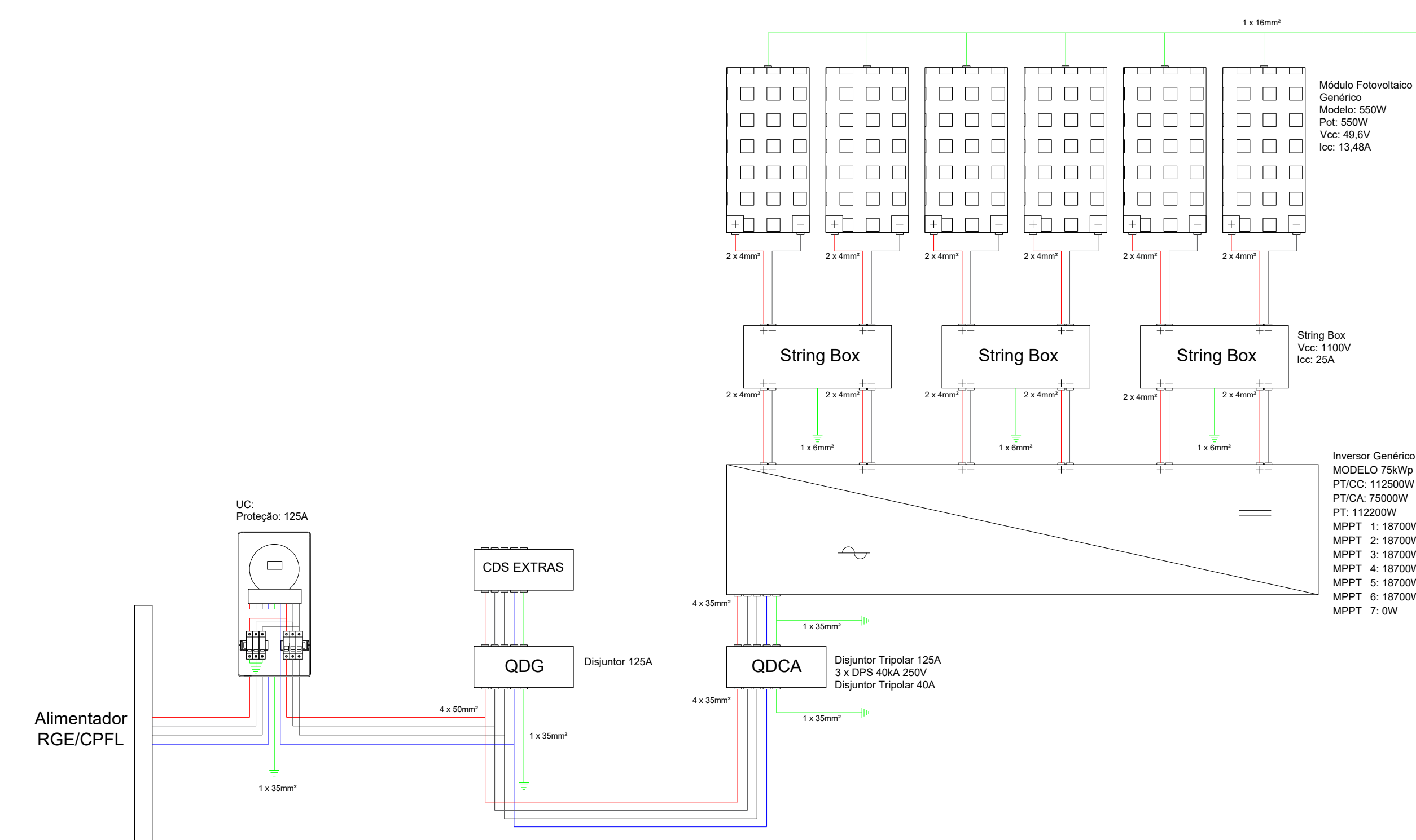
Diagrama Multifilar
