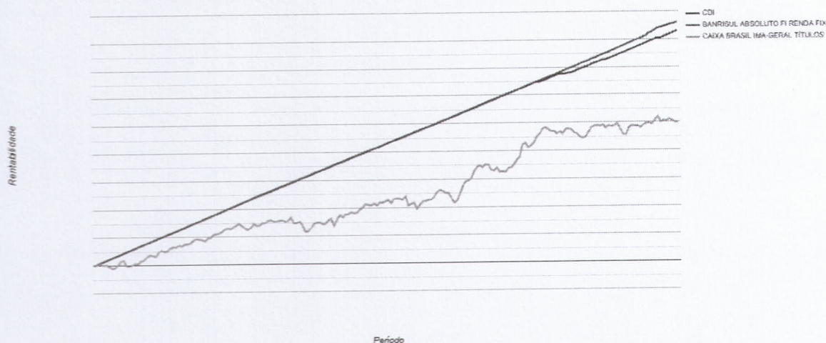
Benchmark - Performance
